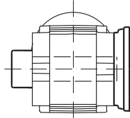
WHF.. Flange-mounted + hollow shaft with keyless shrink disc
