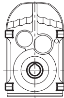
FH..B Foot-mounted (tapped holes) + keyless shrink disc
