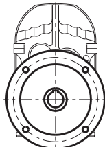
FAF.. B5 flange-mounted + hollow shaft with key
