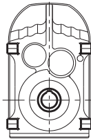
FA..B Foot-mounted (tapped holes) + hollow shaft with key
