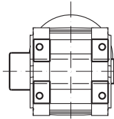
WH..B Foot-mounted + hollow shaft with keyless shrink disc
